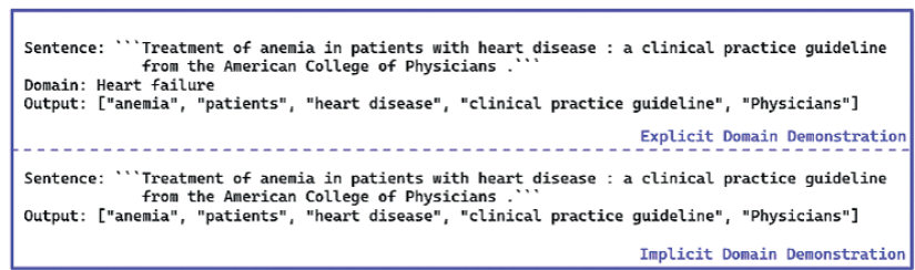
Fig. 3. Explicit vs. implicit in-domain demonstration designed for the ANN version.
