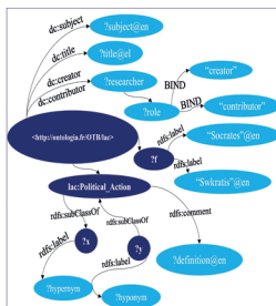
Pic 1. The query graphs visualized
